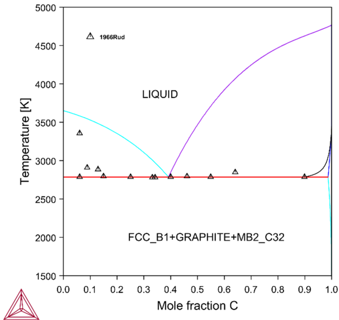
Figure 8: Calculated vertical section of at HfB 2 -C with experimental data from [1966Rud].
