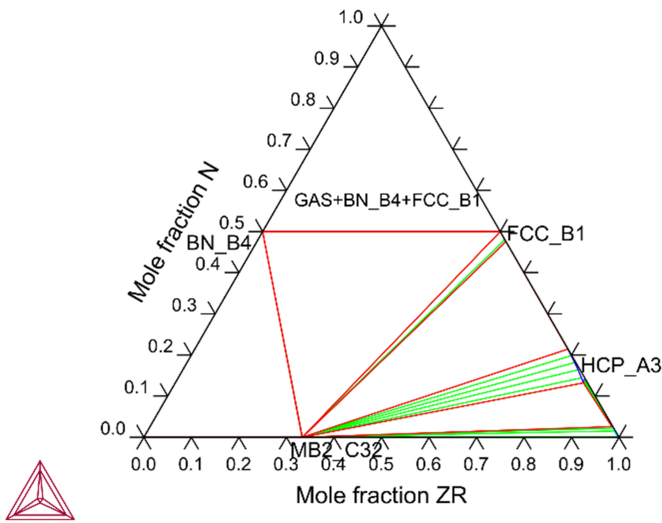
Figure 10: Calculated Zr-B-N isothermal section at 1773 K.
