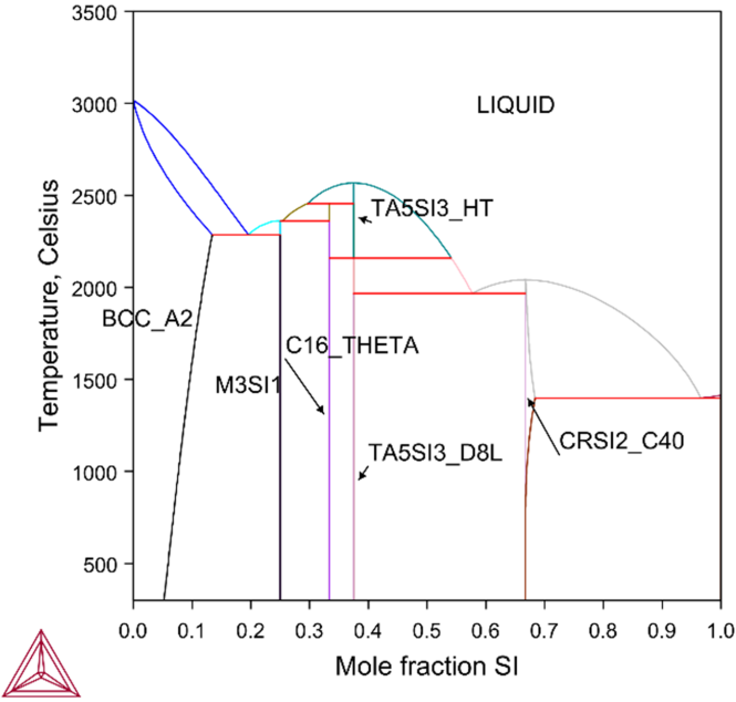
Figure 6: Calculated Ta-Si phase diagram.
