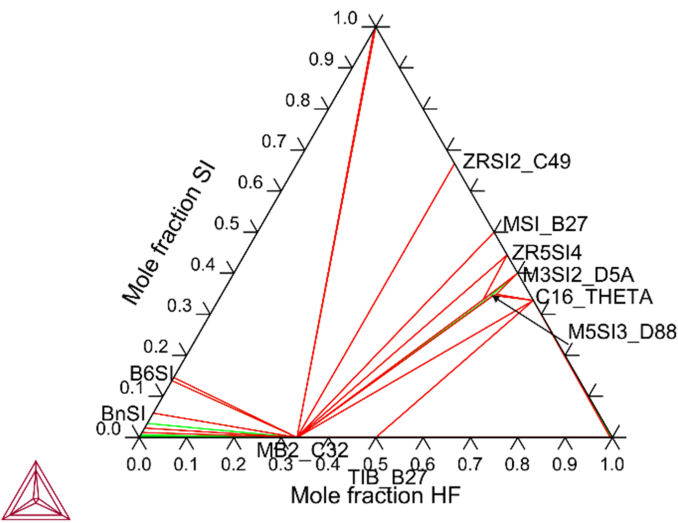
Figure 9: Calculated Hf-Si-B isothermal section at 1573 K.
