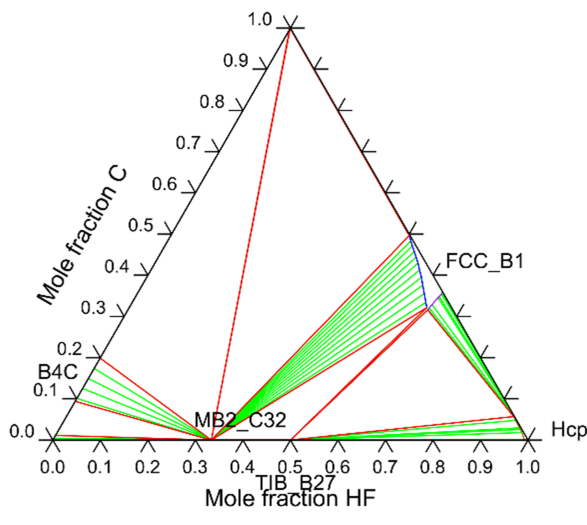
Figure 7: Calculated Hf-B-C isothermal section at 1773 K.
