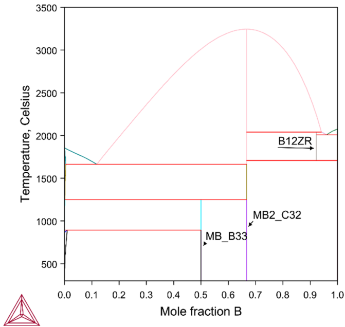
Figure 4: Calculated Zr-B phase diagram.
