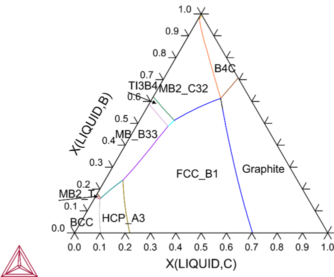
Figure 11: Calculated Ta-B-C liquidus projection.
