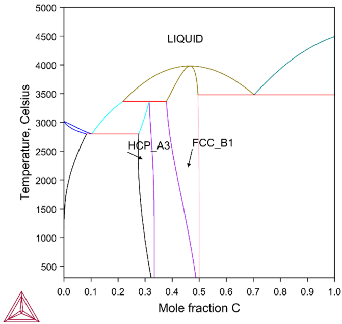
Figure 5: Calculated Ta-C phase diagram.
