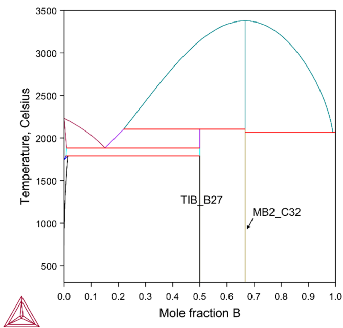
Figure 3: Calculated Hf-B phase diagram.
