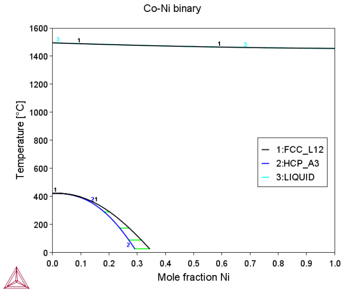
Figure 2: The Co-Ni binary phase diagram.
