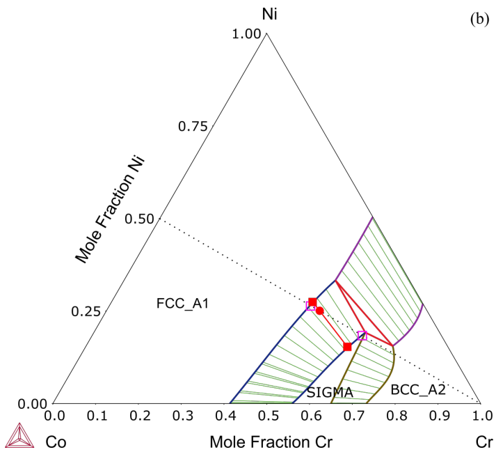
Figure 6: Equilibrium calculation of the extensively studied medium entropy alloy (MEA), the Co-Cr-Ni ternary system. This plot shows an isothermal section at 1200 °C. The alloy composition locates at \text{Co}_{0.25}\text{Ni}_{0.25}\text{Cr}_{0.50} [2018Che].
