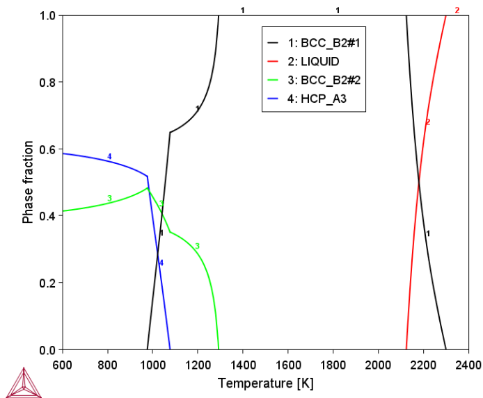
Figure 19: Mole fraction of equilibrium phases at various temperatures in the HfNbTaTiZr equiatomic alloy. The pioneering work of this type of refractory HEA was reported in [2011Sen].
