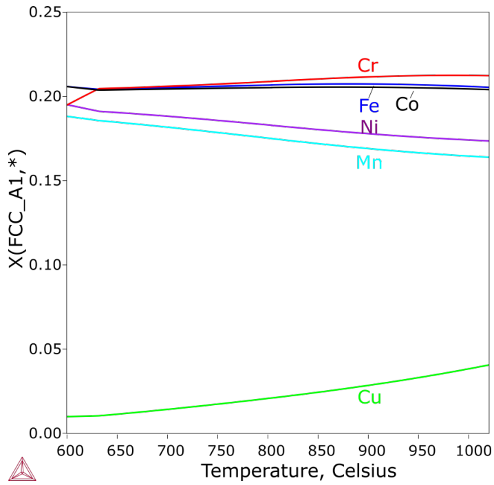
Figure 41: Scheil calculation of the CoCrCuFeMnNi alloy. The composition of the Cu-lean FCC_A1 dendritic phase from the Scheil simulation of CoCrCuFeMnNi.
