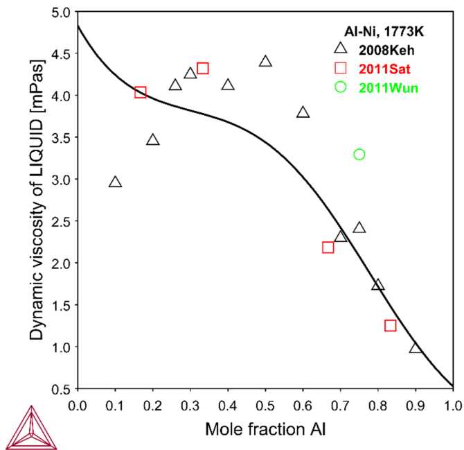
Figure 12: Calculated dynamic viscosity of Al-Ni at 1773 K along with experimental data from [2008Keh; 2011Sat; 2011Wun].
