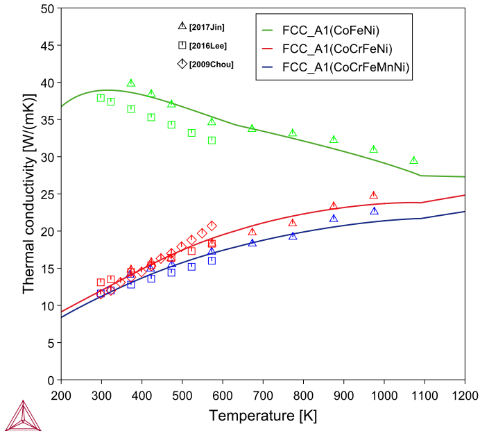
Figure 29: Thermal conductivity of equiatomic FCC medium- and high-entropy alloys at various temperatures. Curves represent calculations while symbols for experimental data from different literature. Each alloy (composition) is assigned a specific color.
