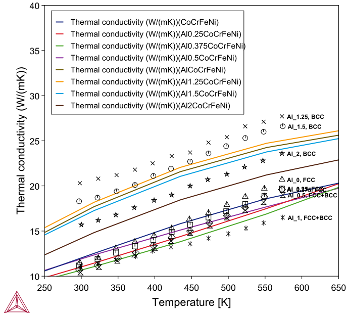
Figure 30: Thermal conductivity of Al_xCoCrFeNi high-entropy alloys at various temperatures. Curves represent (freeze-in) calculations while symbols for experimental data (of as-homogenized alloys at 1373 K) from the literature [2009Chou]. The notation e.g. “Al_1.25, BCC” implies the experimental series for the alloy Al_{1.25}CoCrFeNi with BCC structure.
