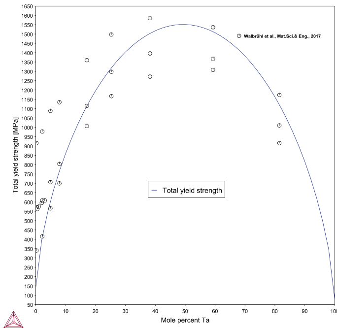
Figure 35: Total yield strength of the Mo-Ta BCC binary alloy in comparison with the experimental data from [2017Wal]. This example is included with Thermo-Calc as a Property Model example named PM_G_06_Yield_Strength_HEA .
