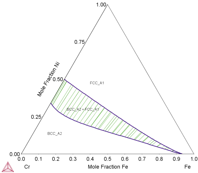
Figure 7: Equilibrium calculation of the Cr-Fe-Ni ternary with an isothermal section at 1300 °C.
