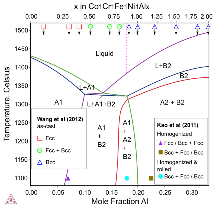
Figure 23: Phase equilibria in the vertical section for \text{CoCrFeNiAl}_x ( 0 < x < 2 ) alloys [2018Che].
