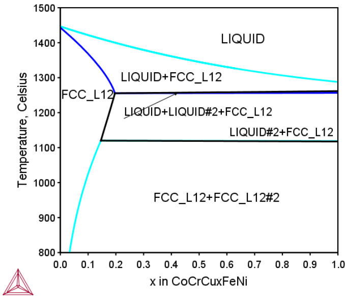
Figure 17: Calculated phase equilibria in the isopleth for the series of the CoCrCu x FeNi quinary alloys, where x=0-1 represents moles of Cu atoms [2017Mao].
