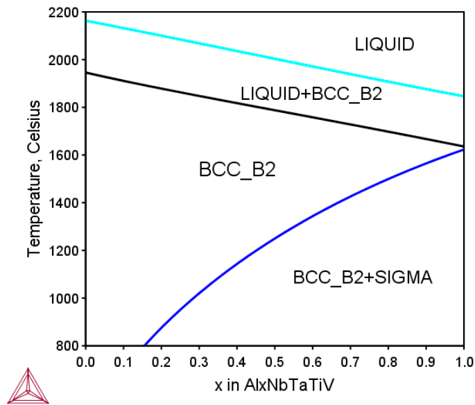
Figure 20: Calculated phase equilibria in the isopleth for the series of the Al x NbTaTiV quinary alloys, where x=0-1 represents moles of atoms of the element Al [2017Mao].
