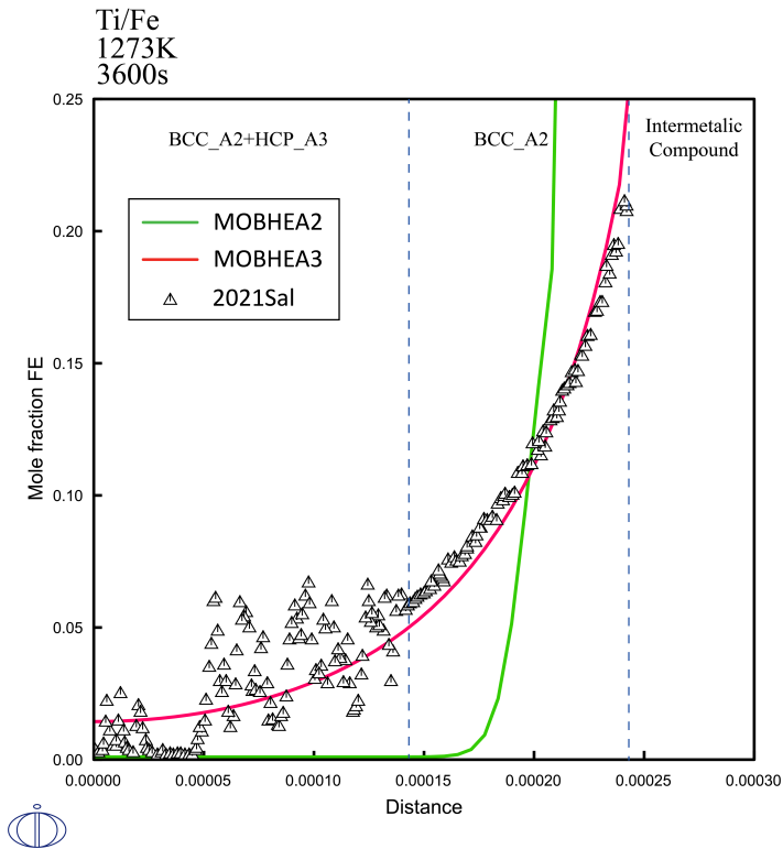
Figure 45: Simulated concentration profiles of Fe in the diffusion couple Fe/Ti annealed after 1 h at 1273 K compared with experimental data [2021Sal].
