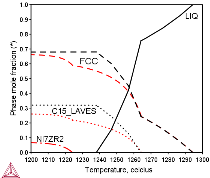
Figure 37: Predicted solid phase mole fractions by equilibrium (black curves) and Scheil simulation (red curves) of the CoCrFeNiZr 0.4 alloy [2017Mao].
