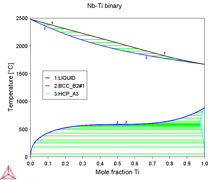
Figure 3: The Nb-Ti binary phase diagram.
