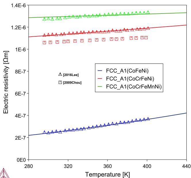
Figure 31: Electrical resistivity of equiatomic FCC medium- and high-entropy alloys at various temperatures. Curves represent calculations while symbols for experimental data from different literature. Each alloy (composition) is assigned a specific color.
