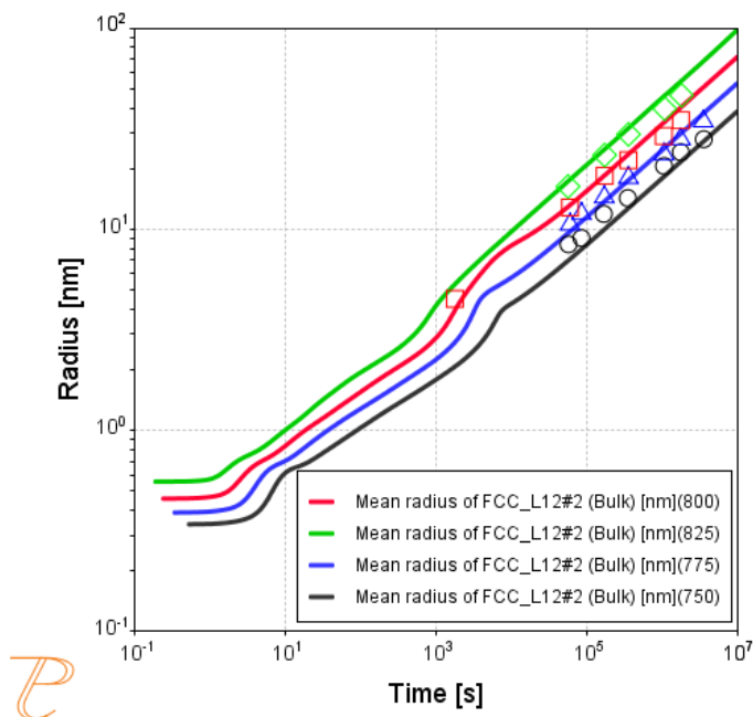
Figure 46: A Precipitation Module (TC-PRISMA) simulation of L1_2 precipitate from the (\text{NiCoFeCr})_{94}\text{Ti}_2\text{Al}_4 HEA matrix at various temperatures. This plot shows the mean radius of the L1_2 precipitates.
