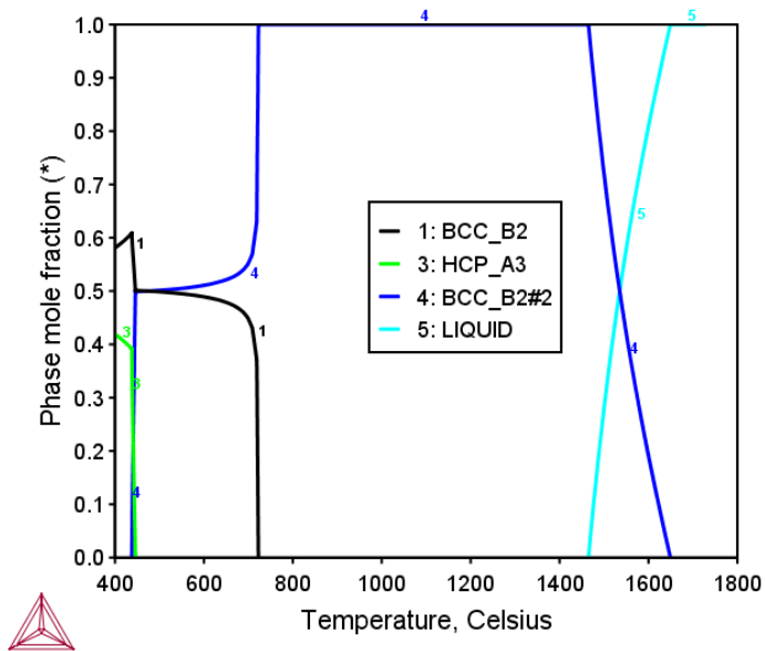
Figure 18: Mole fraction of equilibrium phases at various temperatures in the NbTiVZr equiatomic alloy [2017Mao].
