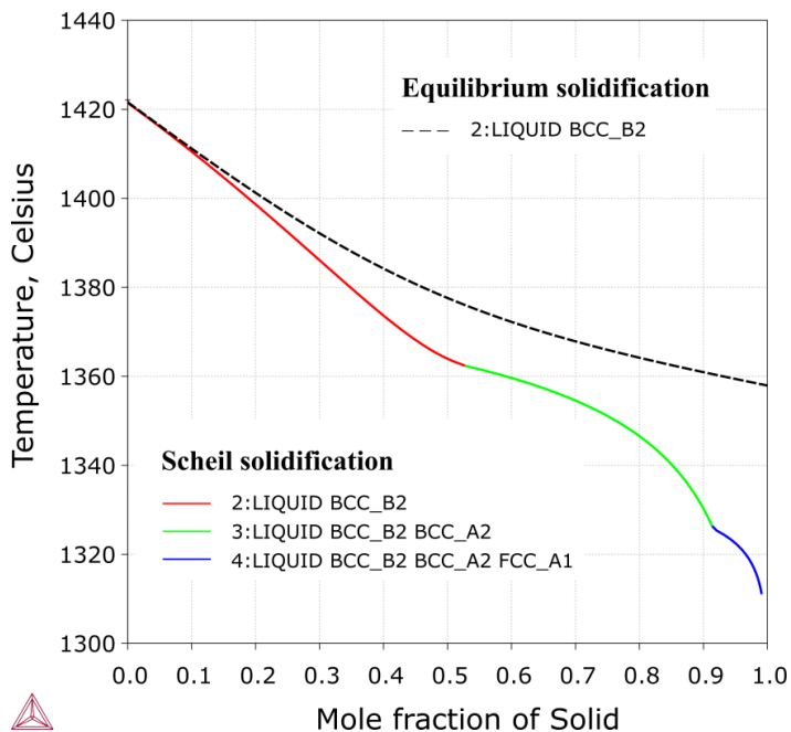
Figure 36: Equilibrium (in dashed line) and Scheil (in solid line) solidification simulations of the \text{CoCrFeNiAl}_{1.1} alloy (21.57 at.% Al) [2018Che].
