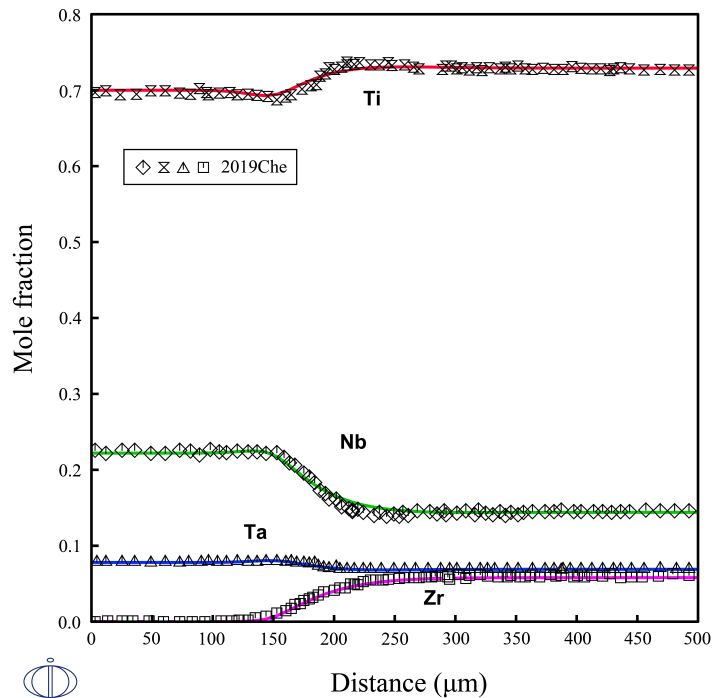
Figure 44: Simulated concentration profiles of diffusion couple Ti-0.222Nb-0.078Ta/Ti-0.144Nb-0.069Ta-0.058Zr with BCC_A2 phase annealed after 64800 s at 1373 K compared with the experimental data [2019Che].
