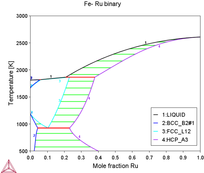
Figure 4: The Fe-Ru binary phase diagram.
