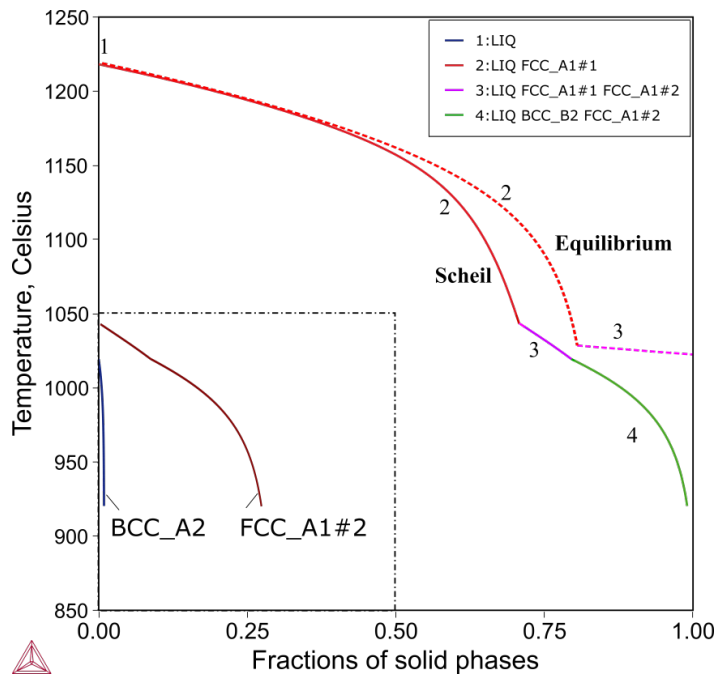
Figure 40: Scheil and equilibrium calculations of the CoCrCuFeMnNi alloy. Total and individual solid phase fraction from the Scheil simulation (in solid lines) and equilibrium calculation (in dashed lines) of CoCrCuFeMnNi. The phase fractions of the minor phases (FCC_A1#2 and BCC_A2) are imposed and enclosed with the dashed-dotted lines.
