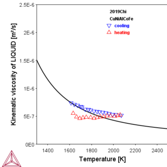
Figure 33: Calculated kinematic viscosity of equiatomic Cu-Ni-Al-Co-Fe alloy along with experimental data from [2019Chi].
