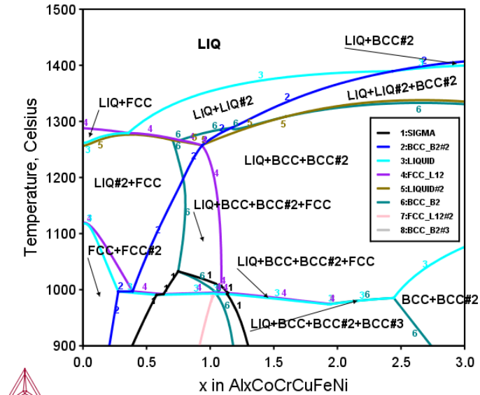
Figure 24: Calculated phase equilibria in the isopleth for the series of the Al x CoCrCuFeNi senary alloys, where x=0-3 represents moles of atoms of the element Al [2017Mao].
