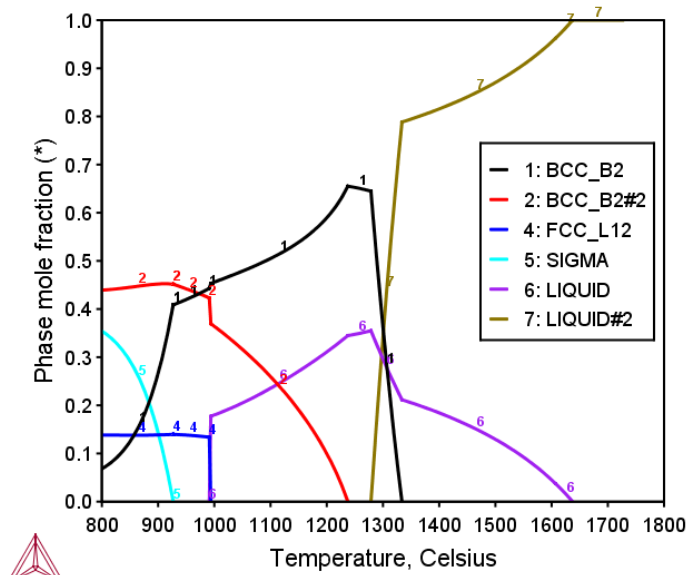
Figure 25: Calculated mole fraction of equilibrium phases at various temperatures in the AlCoCrCuFeNiV septenary alloy with equiatomic ratio [2017Mao].
