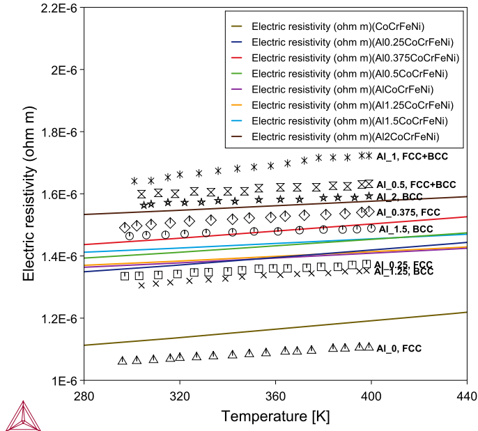
Figure 32: Electrical resistivity of Al_xCoCrFeNi high-entropy alloys at various temperatures. Curves represent (freeze-in) calculations while symbols for experimental data (of as-homogenized alloys at 1373 K) from the literature [2009Chou]. The notation e.g. “Al_0.375, FCC” implies the experimental data for the alloy Al_{0.375}CoCrFeNi with single FCC phase.
