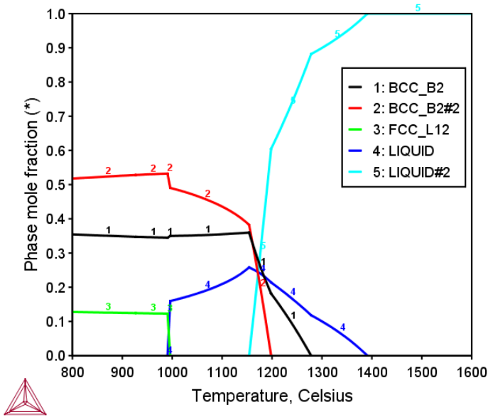
Figure 26: Calculated mole fraction of equilibrium phases at various temperatures in the AlCoCrCuFeNiTiV octonary alloy with equiatomic ratio [2017Mao].
