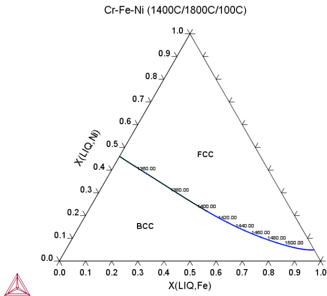
Figure 8: Equilibrium calculation of the Cr-Fe-Ni ternary showing a liquidus surface projection. The temperature (°C) value is plotted along the monovariant reaction curve. The primary phase shifts from BCC in Cr-corner to FCC in Ni-corner.
