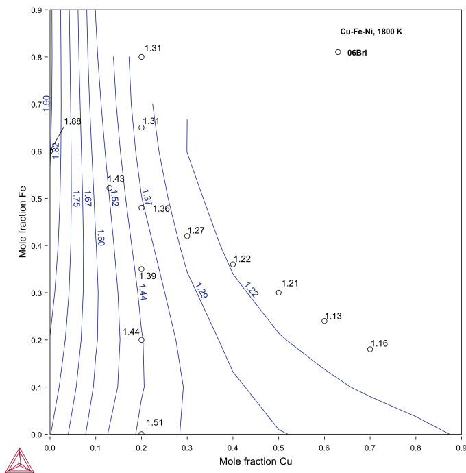
Figure 34: Calculated surface tension of ternary Cu-Fe-Ni liquid at 1800 K in comparison with experimental data of [2006Bri].
