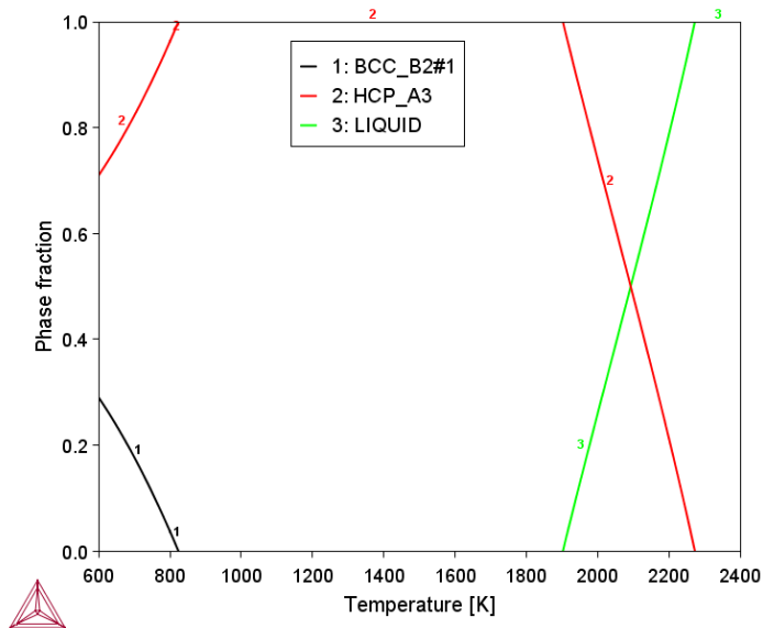
Figure 21: Mole fraction of equilibrium phases at various temperatures in the CoFeReRu equiatomic alloy. The experimental validation is reported in [2016Gao].
