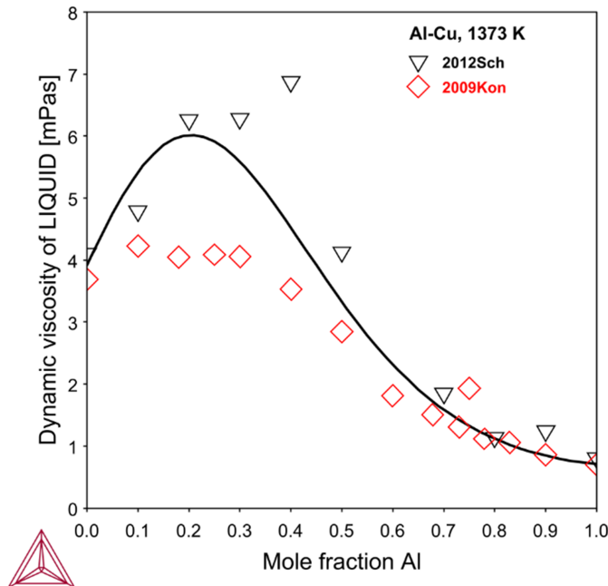
Figure 11: Calculated dynamic viscosity of Al-Cu at 1373 K along with experimental data from [2009Kon; 2012Sch].
