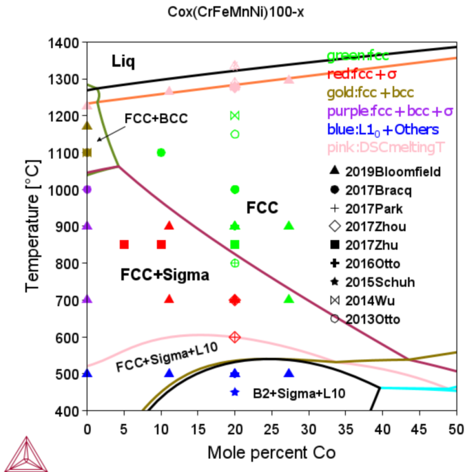
Figure 16: Calculated phase equilibria in the isopleth of \text{Co}_x(\text{CrFeMnNi})_{100-x} , where x represents at% of Co. In the plot, symbols represent experimentally observed phases. These are coded in color for different phase assemblages, e.g. green for single FCC, and red for FCC+Sigma two-phase coexists. Different symbols represent different experimental work. Filled and empty symbols stand for long ( \geq 24 h) and short ( < 24 h) annealing, respectively.
