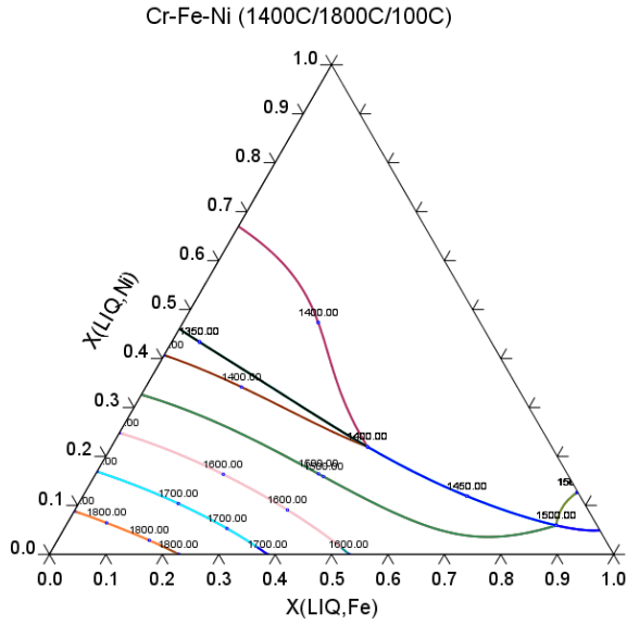
Figure 9: Equilibrium calculation of the Cr-Fe-Ni ternary with a liquidus projection overlapping with series of isothermal sections of the Cr-Fe-Ni ternary.
