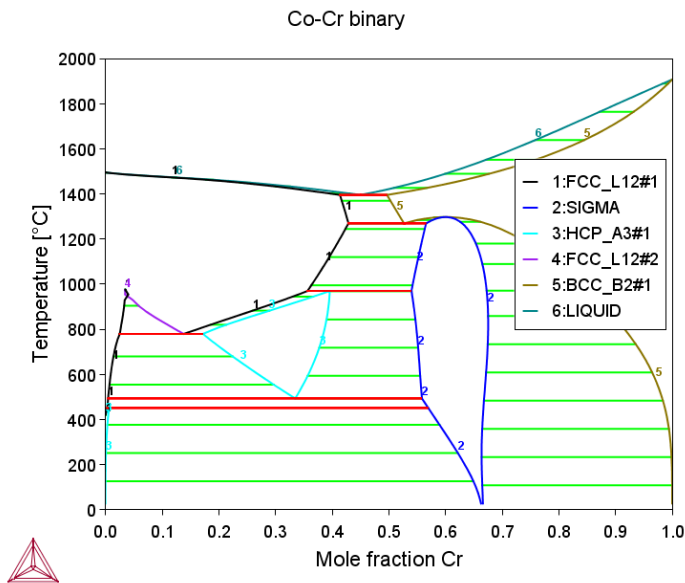
Figure 1: The Co-Cr binary phase diagram.
