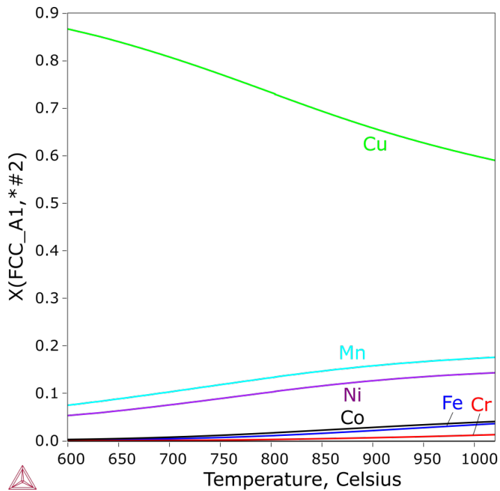
Figure 42: Scheil calculation of the CoCrCuFeMnNi alloy. The composition of the Cu-rich FCC_A1 interdendritic phase from the Scheil simulation of CoCrCuFeMnNi.
