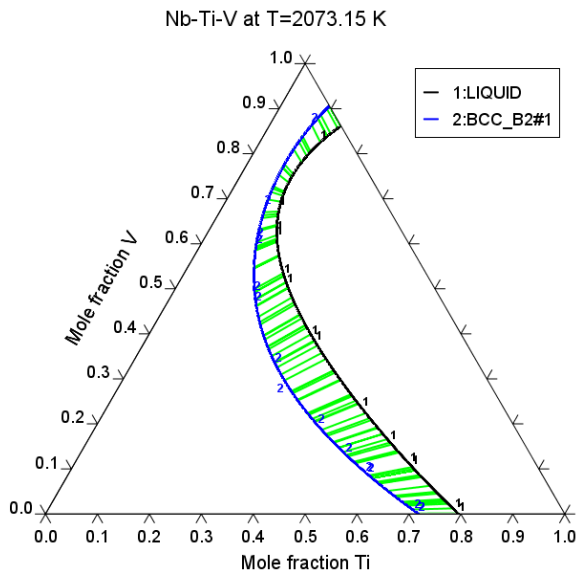
Figure 10: Isothermal section at 1800 °C of the Nb-Ti-V ternary.
