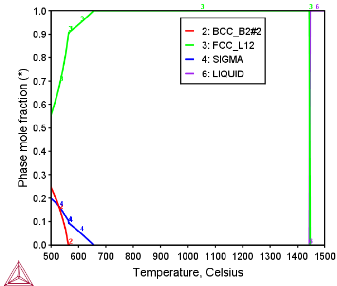
Figure 14: Mole fraction of equilibrium phases at various temperatures in the CoCrFeNi equiatomic alloy [2017Mao].
