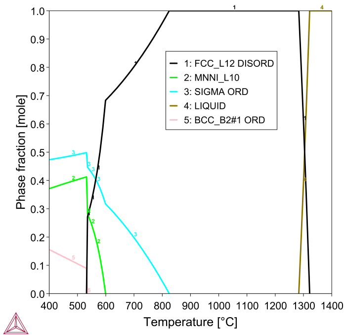
Figure 15: Mole fraction of equilibrium phases at various temperatures in the CoCrFeMnNi equiatomic alloy, a.k.a. the Cantor alloy [2004Can].
