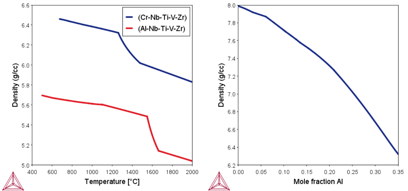
Figure 28: Calculated density of HEAs. (a) Density of CrNbTiVZr and AlNbTiVZr HEAs at various temperatures. The measured room temperature density is 6.57 g/cc for CrNbTiVZr [2013Sen] and 5.79 g/cc for AlNbTiVZr [2015Ste]. (b) Density of Al x CoCrFeNi HEAs at 400°C.
