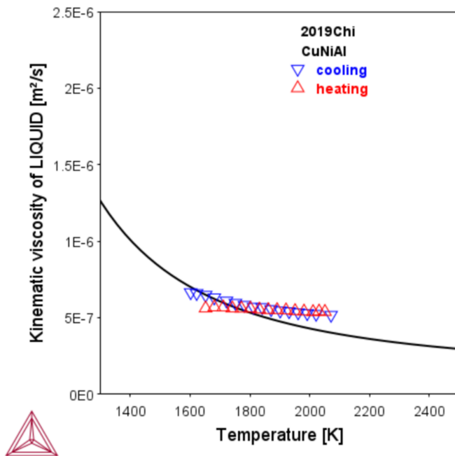
Figure 13: Calculated kinematic viscosity of equiatomic Cu-Ni-Al alloy along with experimental data from [2019Chi].
